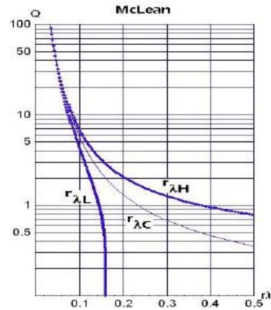
Figure 11: McLean’s limit. Note how r\lambda_L converges in a well-behaved manner to the “radiansphere:”
