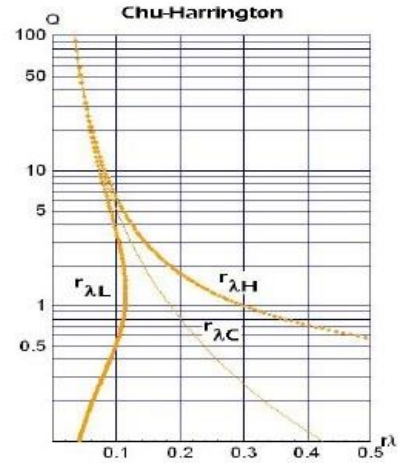
Figure 10: The Chu-Harrington limit. Note the non-physical behavior of r\lambda_L .
