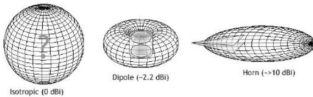
Figure 2: An isotropic antenna (left) has a gain of 0 dBi by definition. A small dipole antenna (center) typically has a gain of about 2.2 dBi, and a horn antenna (right) may have a gain of 10 dBi or more.
