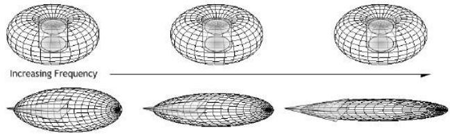
Figure 7: The pattern of a constant gain antenna remains fixed with increasing frequency (top), while the pattern of a constant aperture antenna narrows and gain increases with increasing frequency.
