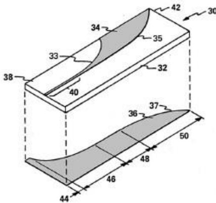
Figure 4: The continuously tapered slot horn elements of Nester (gray colorization on elements added).
